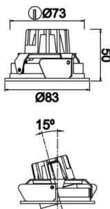
Technical Drawing
