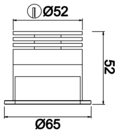
Technical Drawing
