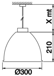
Technical Drawing
