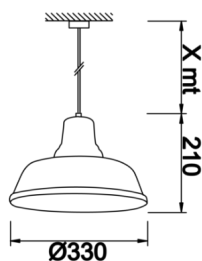
Technical Drawing
