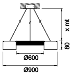
Technical Drawing
