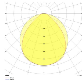
Photometric Curve
