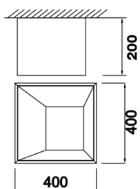
Technical Drawing
