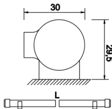
Technical Drawing
